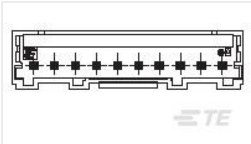
TE Part #1971032-7 7pos header assembly for gic 2.0 ev
