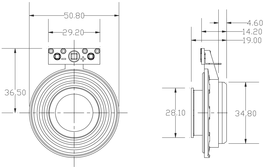
Figure 2. Nominal dimensions
