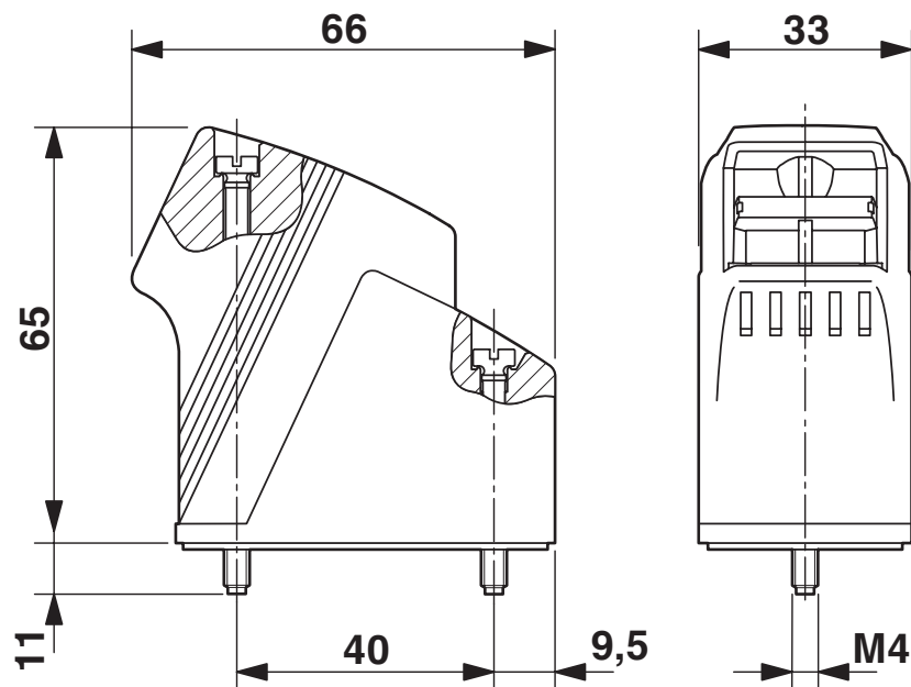
Dimensional drawing
