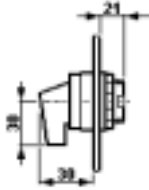
Switch- and potentiometer actuator *
