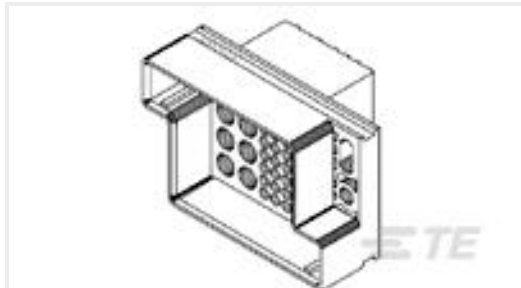
TE Part #194243-1 AMPOWER HOUSING,RCPT,43 POS
