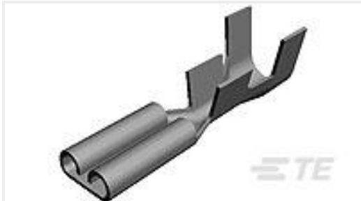
TE Part #170213-2 250 FASTON,REC.,18-14 AWG,TPBR
