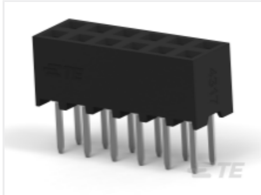
TE Part # 1-2314821-4 14P,2MM,B-B,REC,DRVT,2.7,0.38AU,TB
