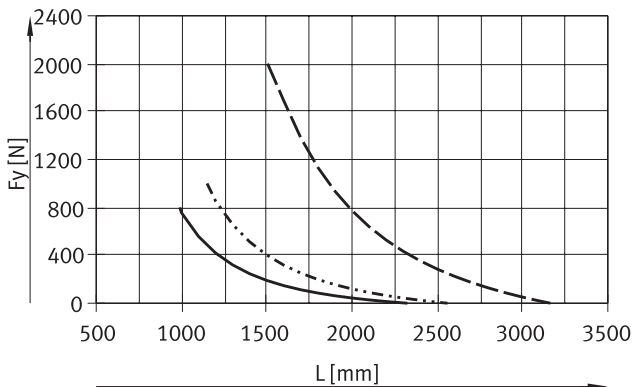
Force Fy
