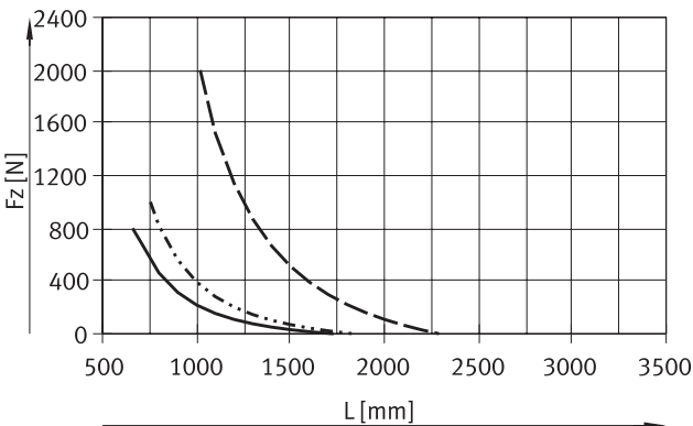
Force Fz
