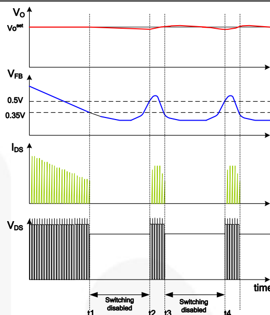
Figure 22. Burst-Mode Operation
