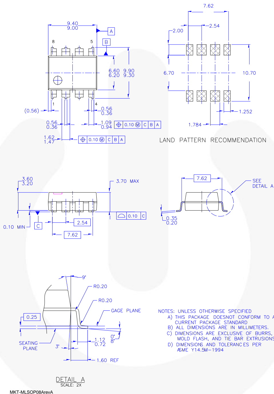
Figure 25.8-Lead, 300μm Wide, Surface Mount Package (LSOP)
