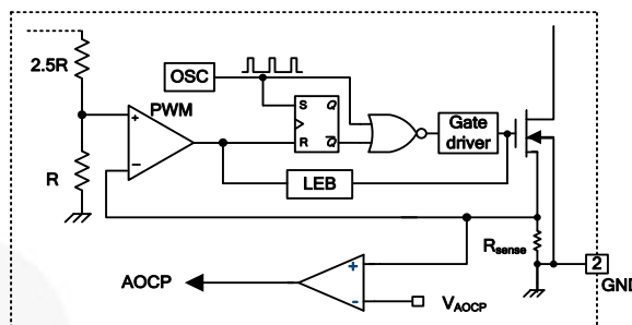
Figure 19. Abnormal Over-Current Protection
