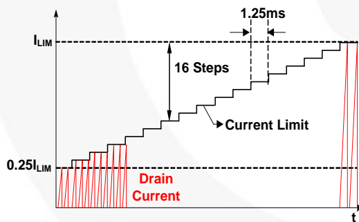
Figure 21. Internal Soft-Start
