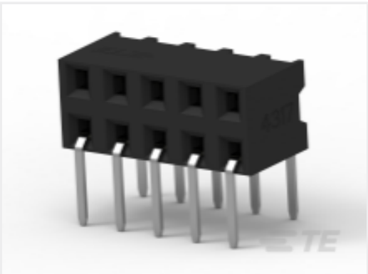
TE Part # 1-2307722-4 14P,2MM,B-B,REC,DRHZ,2.8,0.76AU, TB
