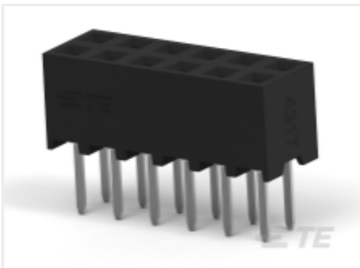
TE Part # 1-2307785-4 14P,2MM,B-B,REC,DRV,2.0,0.76AU, TR,W/CAP
