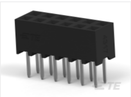
TE Part # 1-2314826-4 14P,2MM,B-B,REC,DRV,2.7,0.76AU, TB,W/CAP
