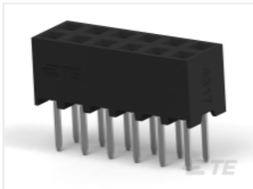
TE Part # 1-2307787-4 14P,2MM,B-B,REC,DRV,3.2,0.76AU, TUBE
