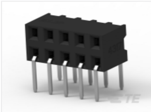
TE Part # 1-2307723-4 14P,2MM,B-B,REC,DRHZ,3.4,0.76AU, TUBE
