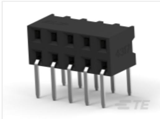
TE Part # 1-2314926-4 14P,2MM,B-B,REC,DRHZ,2.8,0.76AU,TR
