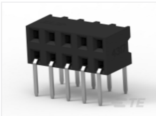
TE Part # 1-2314918-4 14P,2MM,B-B,REC,DRHZ,2.1,0.76AU, TB
