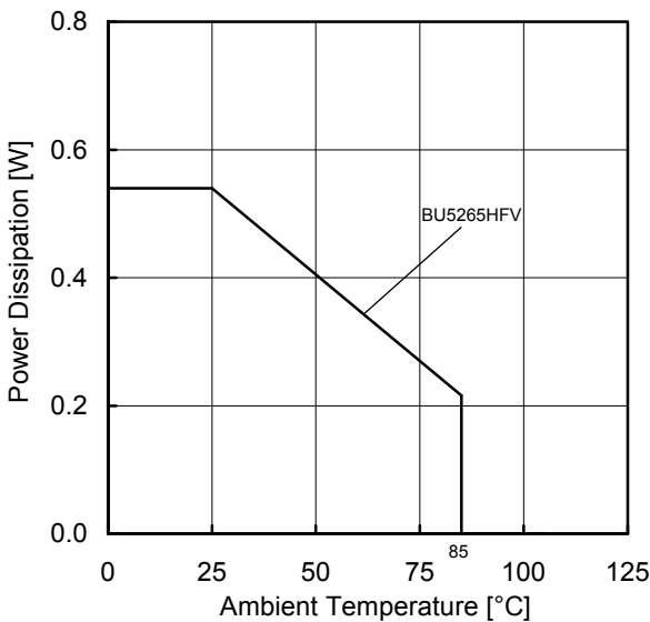
(c) BU5265HFV
