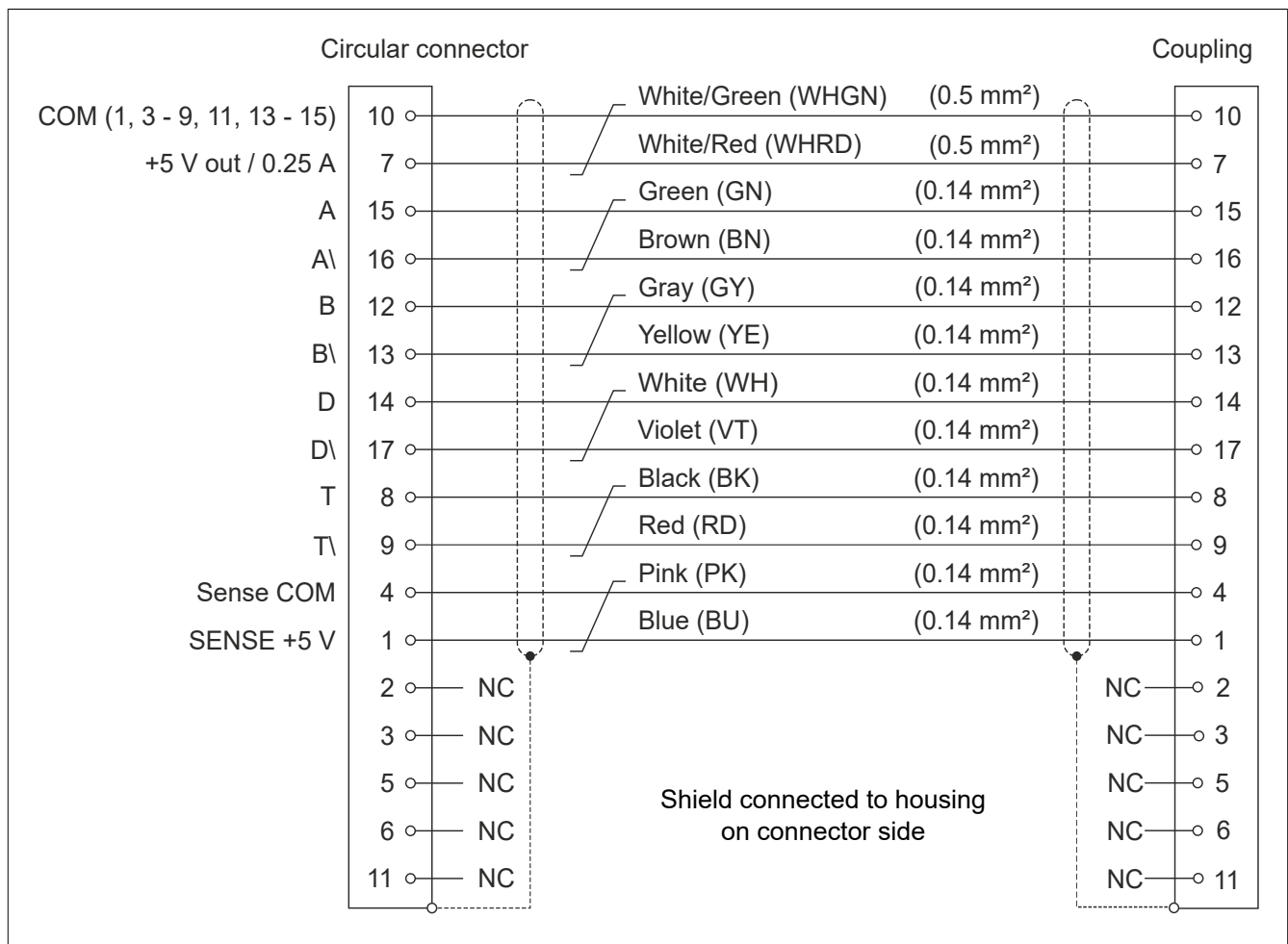
Figure 1: 8BCE cable extension - Cable diagram
