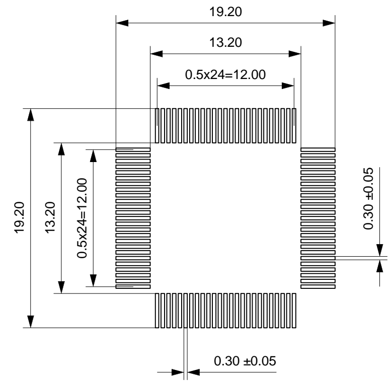
Size of QFP pad Scale 3:1
