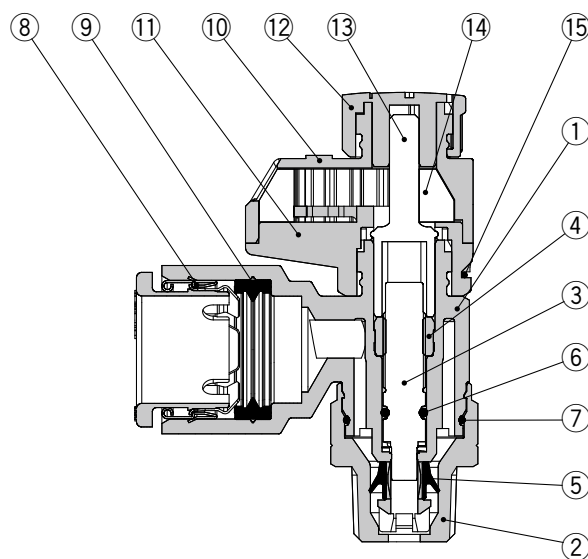
Meter-out type
