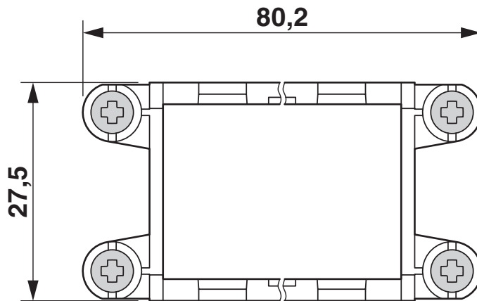
Dimensional drawing
