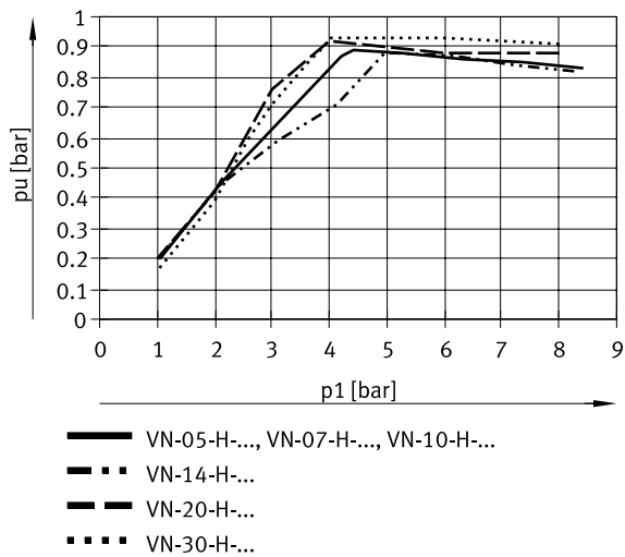
Vacuum p_u as a function of operating pressure p_1 – high vacuum (VN-05/07/10/14/20/30-H)
