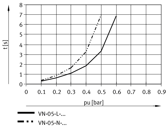
Evacuation time t as a function of vacuum p_u for 1 l volume at 6 bar operating pressure – high suction rate (VN-05-L/N)
