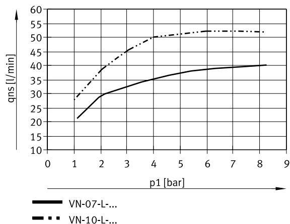
Suction rate q_{ns} (against atmosphere) as a function of operating pressure p_1 – high suction rate (VN-07/10-L)
