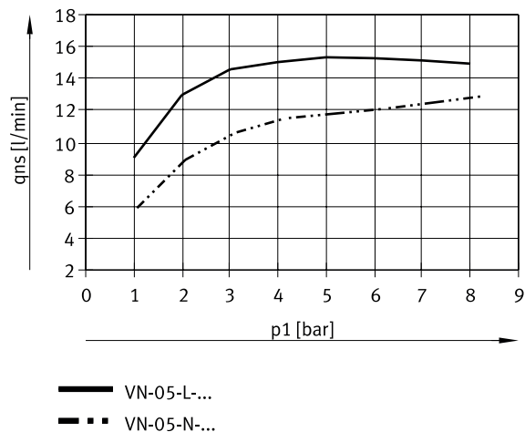
Suction rate q_{ns} (against atmosphere) as a function of operating pressure p_1 – high suction rate (VN-05-L/N)
