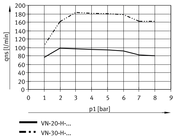
Suction rate q_{ns} (against atmosphere) as a function of operating pressure p_1 – high vacuum (VN-20/30-H)
