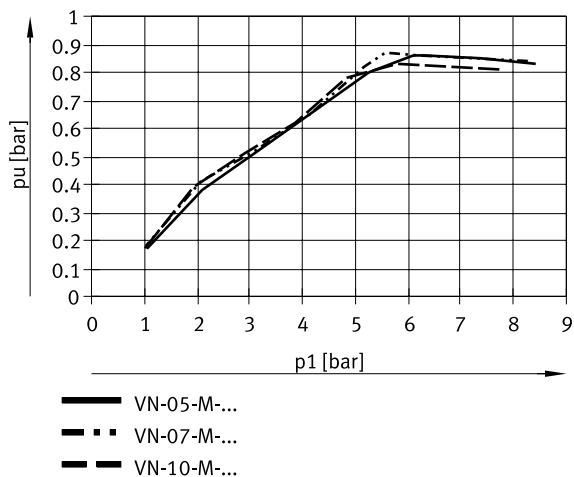
Vacuum p_u as a function of operating pressure p_1 – high vacuum (VN-05/07/10-M)
