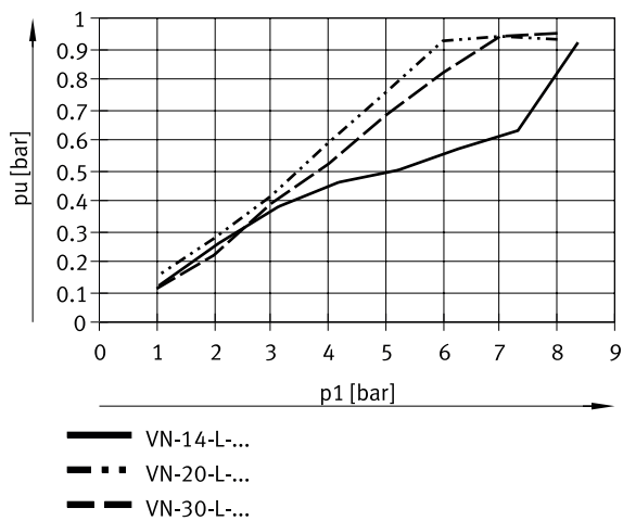
Vacuum p_u as a function of operating pressure p_1 – high suction rate (VN-14/20/30-L)
