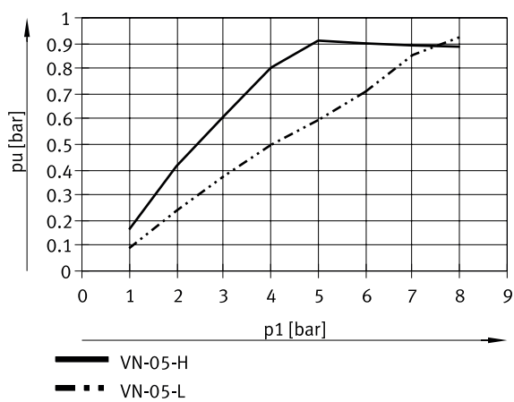
Vacuum p_u as a function of operating pressure p_1 – high vacuum/high suction rate (VN-05-H/L-...-P)
