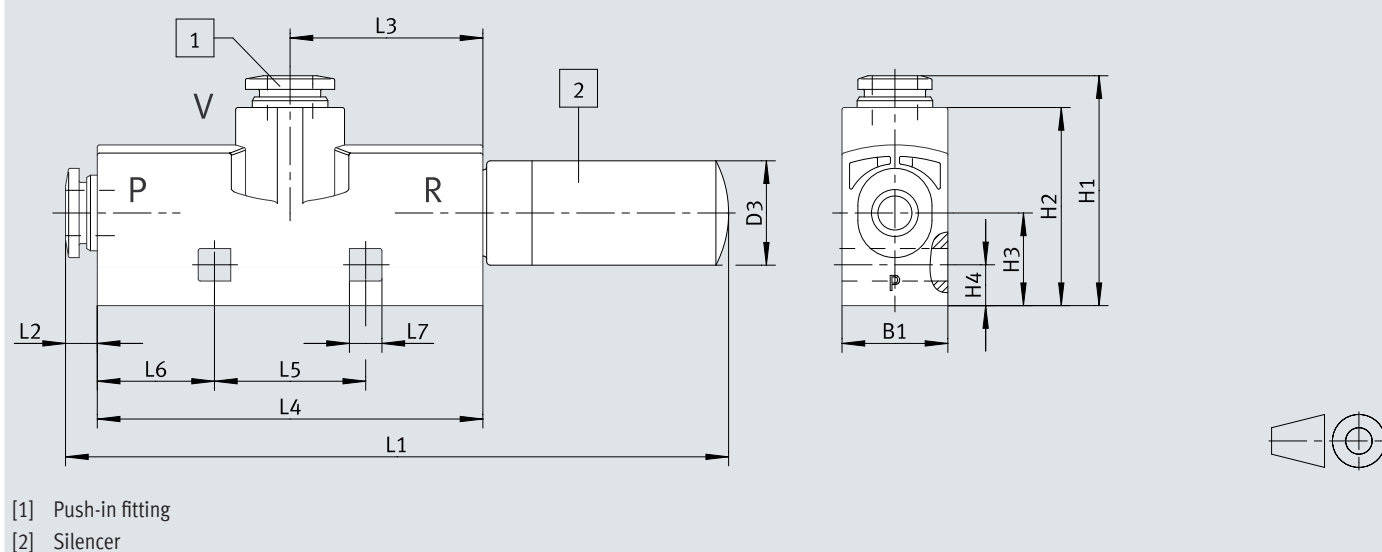
Dimensions – T-shape/standard, VN-...-T...-PQ...-VQ...-RO...
