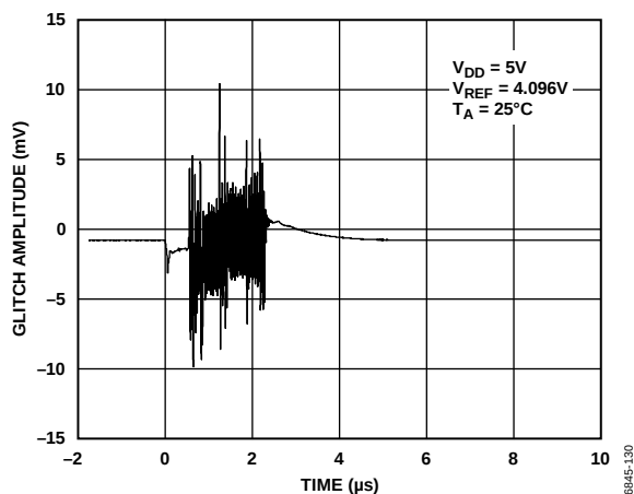
Figure 30. Analog Crosstalk
