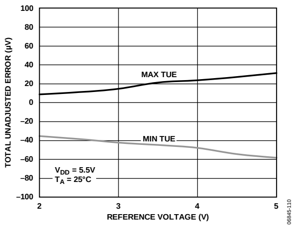
Figure 9. Total Unadjusted Error vs. Reference Input Voltage
