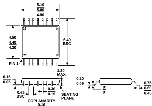
Figure 50. 16-Lead Thin Shrink Small Outline Package [TSSOP] (RU-16) Dimensions shown in millimeter
