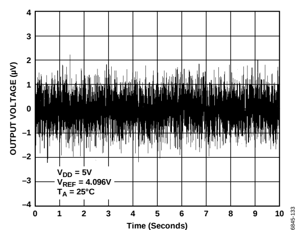
Figure 33. 1/f Noise
