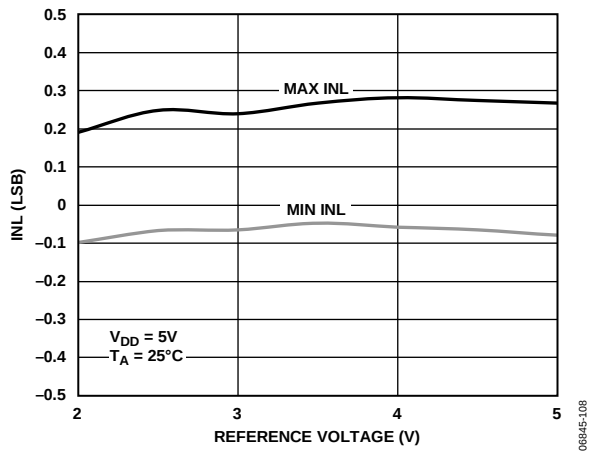
Figure 7. INL vs. Reference Input Voltage
