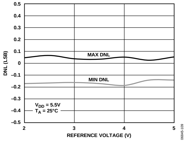
Figure 8. DNL vs. Reference Input Voltage
