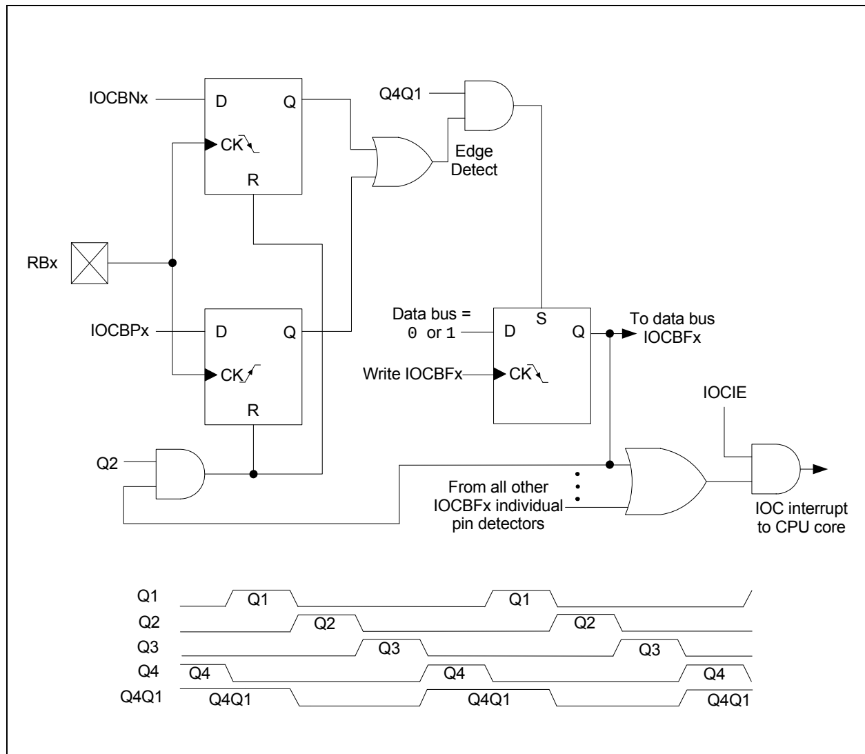
FIGURE 8-1: INTERRUPT LOGIC
