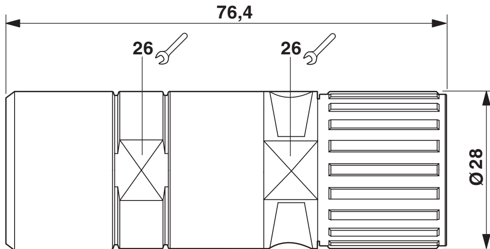
Dimensional drawing
