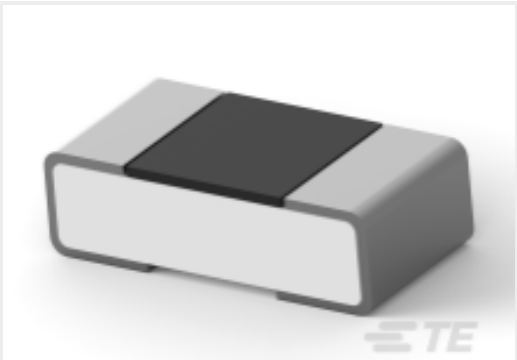
TE Part #6-2176363-6 RQ 0402 2K05 0.1% 10PPM 5K RL
