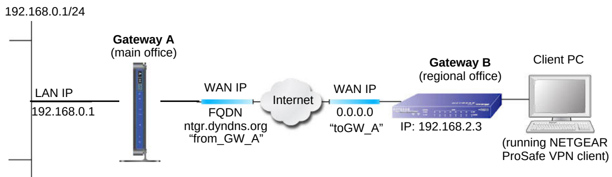
Figure 64. Telecommuter example
