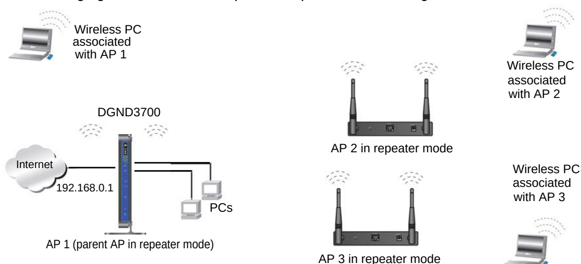
Figure 54. Repeater mode
