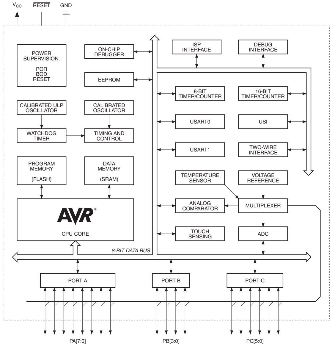
Figure 2-1. Block Diagram
