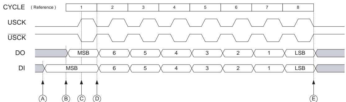
Figure 15-3. Three-wire Mode, Timing Diagram
