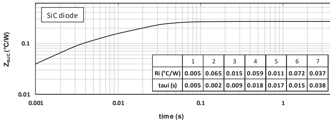
Figure 1-20. Maximum thermal impedance
