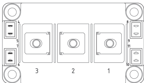
Figure 2. Pinout Location
