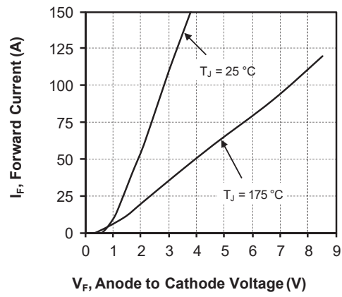
Figure 1-21. Forward Current vs Forward Voltage
