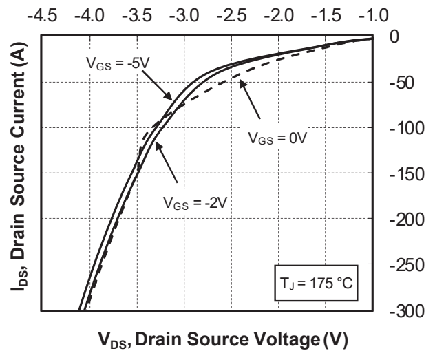
Figure 1-19. Drain Source Voltage Characteristics, T_J = 175\text{ }^\circ\text{C}
