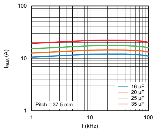
Maximum I_{\text{RMS}} current as function of frequency, based T_A + 85^\circ\text{C} , \Delta t = +15^\circ\text{C} (typical curve)
