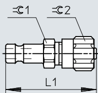
Dimensions – Quick coupling plug KS2, quick connector
