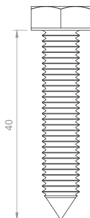
M10x40 SIDE VIEW
