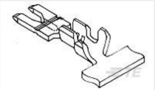
TE Part #281622-2 MAG-MATE TAB STD SNPL
