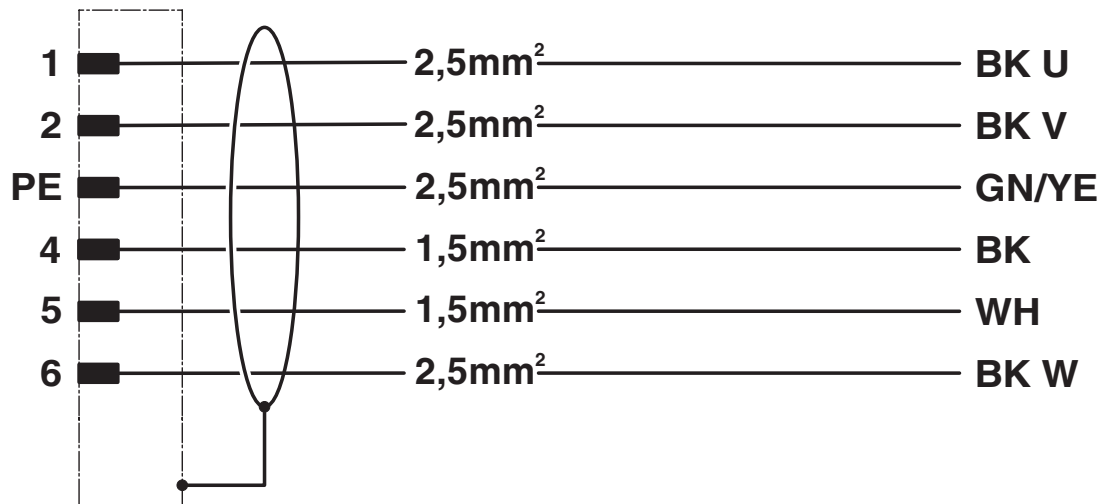
Contact assignment of M23 plugs/sockets
