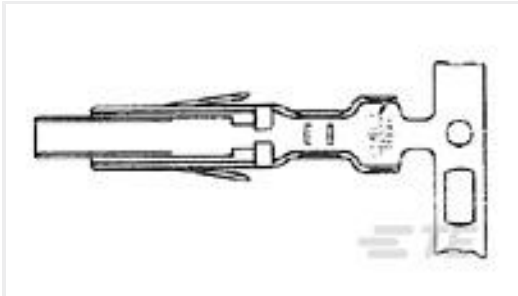
TE Part #1703111-1 CONTACT FOR DRAWER CONN
