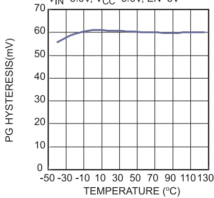
PG Hysteresis vs. Temperature
