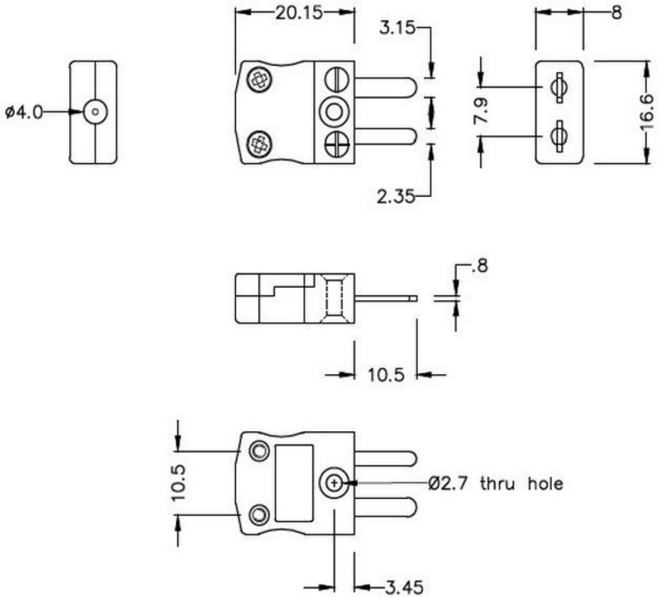
Miniature in-line Plug (dimensions in mm)
