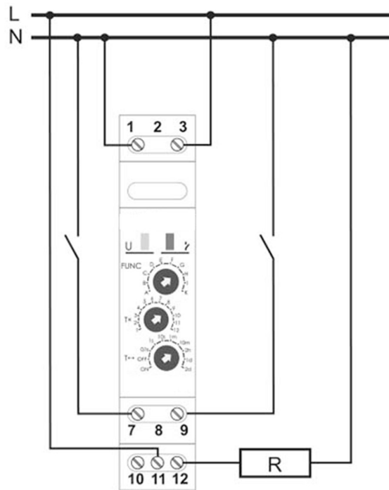
Example of connection with N control signals
