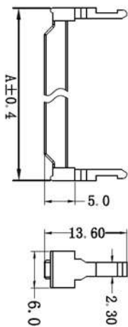
A TYPE Three Piece SR P/N: D2553WVC-2NP-P0BKGI
