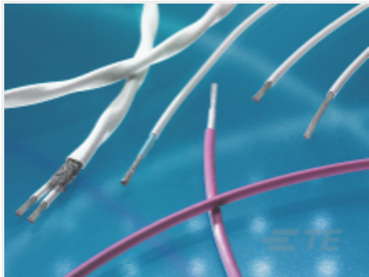
TE Part #CAT-55PC-TC-2T22 2 Core Twisted Pair Cable: Tin Coated Copper Cable, 22 AWG
