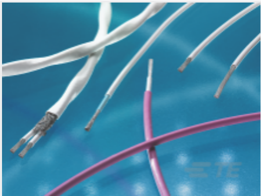
TE Part #CAT-55PC-TC-2T20 2 Core Twisted Pair Cable: Tin Coated Copper Cable, 20 AWG
