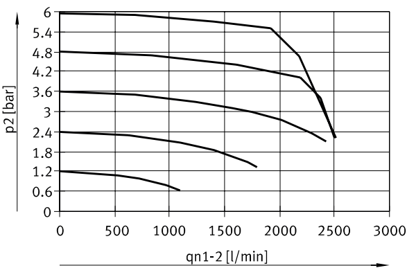
Flow rate q_n from 1 -> 2 as a function of excess output pressure p_2 , VPPM-8L/F-...-0L6H-... (6 bar)
