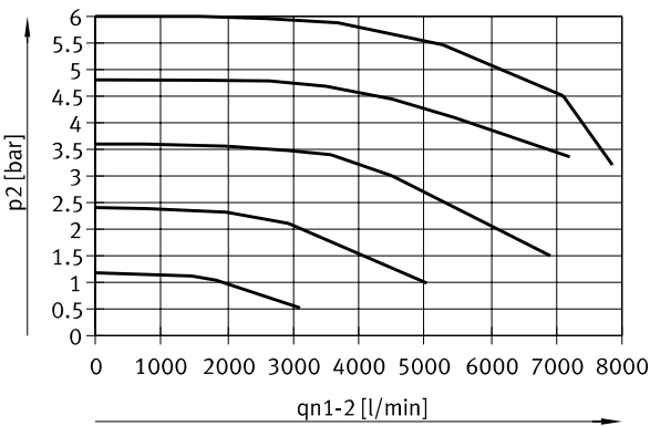
Flow rate q_n from 1 -> 2 as a function of excess output pressure p_2 , VPPM-12L-...-0L6H-... (8 bar)
