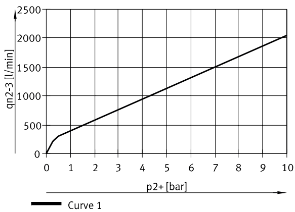
Flow rate q_n from 2 -> 3 as a function of excess output pressure p_2 , VPPM-8F/8TA-...-0L10H-... (10 bar)
