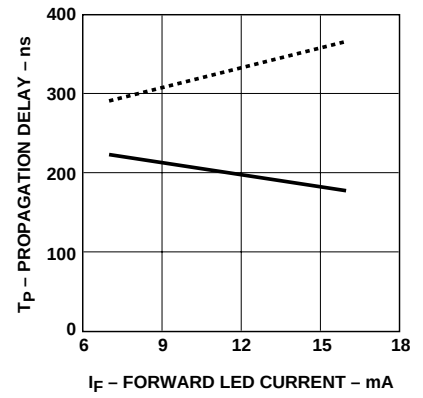
Figure 9. Propagation delay vs. I_F .
