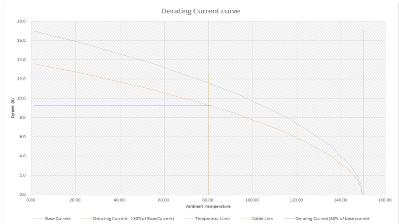
Figure 2: Derating curve 6-pin, 9.3A (angled/ straight)
