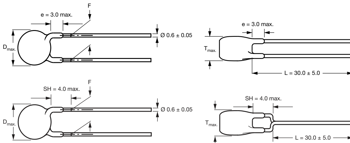
Capacitors with 10.0 mm or 12.5 mm lead spacing
