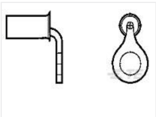
TE Part #321262 TERM, SOLIS, RT, 22-16, #6, 90 BEND
