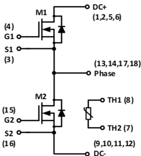
Figure 1. NXH015P120M3F1PTG Schematic Diagram
