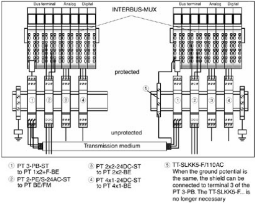
Connecting M-UFB IBS-MUX to the field multiplexer
