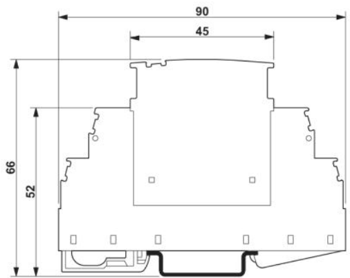
The figure shows the complete module consisting of a base element and connector
