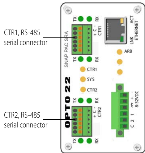
Controller-to-Arbiter Wiring
