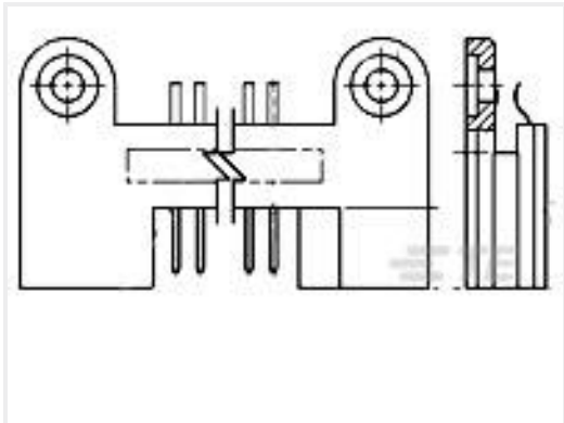
TE Part #1-530785-0 BOX PIN HDR ASSY 70 PS 075 CL
