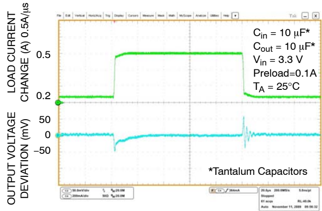
Figure 31. Load Transient Response – V_{out} = 5.0\text{ V}
