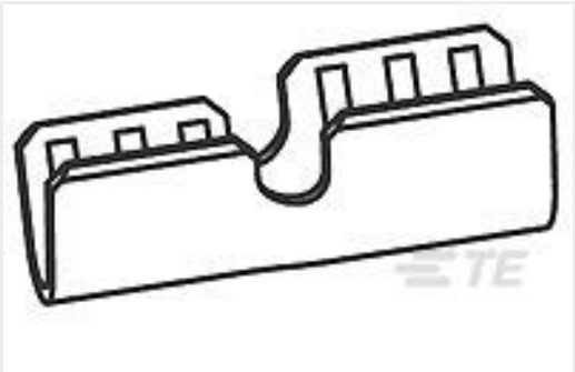
TE Part #61021-1 SPLICE 18-16 AWG .0126 NPST
