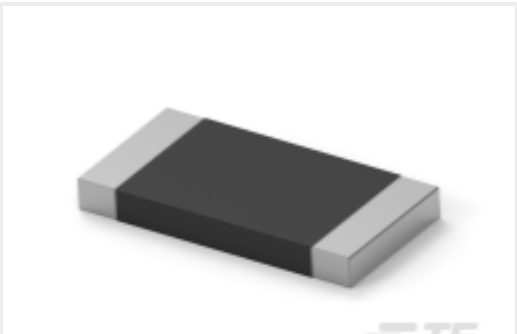
TE Part #6-2176422-2 TLRP 2512 3.0W R033 1% 50PPM 4K RL
