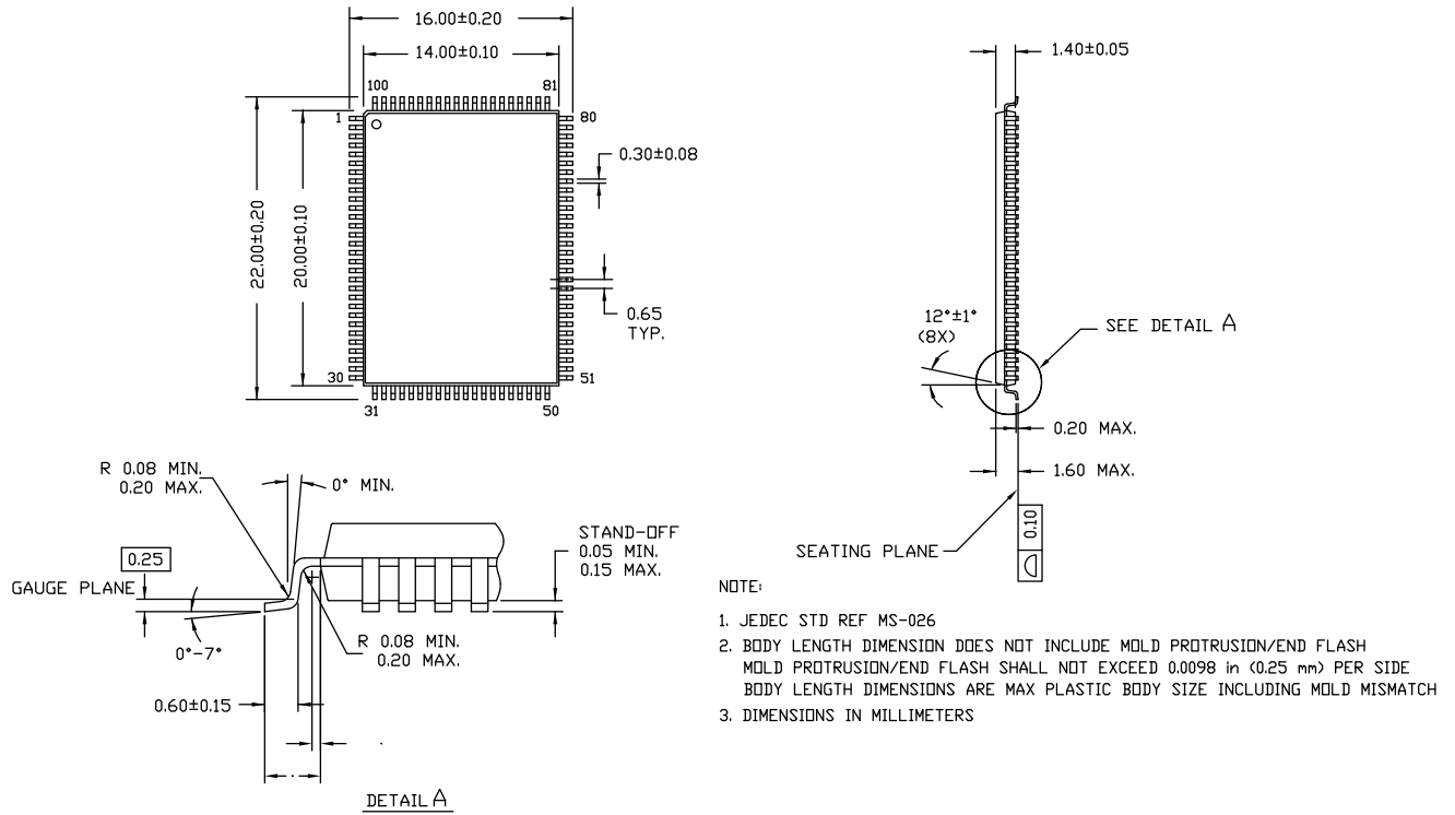
Figure 6. 100-pin TQFP (14 × 20 × 1.4 mm) A100RA Package Outline, 51-85050
