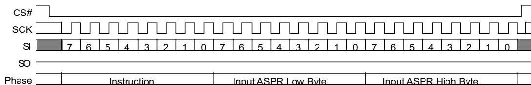
Figure 109. ASPP (2Fh) Command
