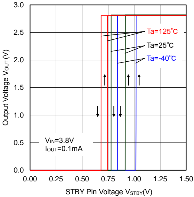
Figure 32. STBY Threshold
