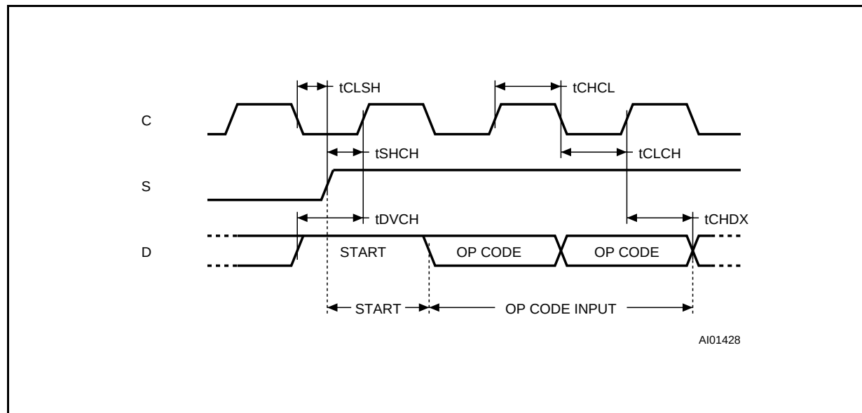
Figure 4. Synchronous Timing, Start and Op-Code Input
