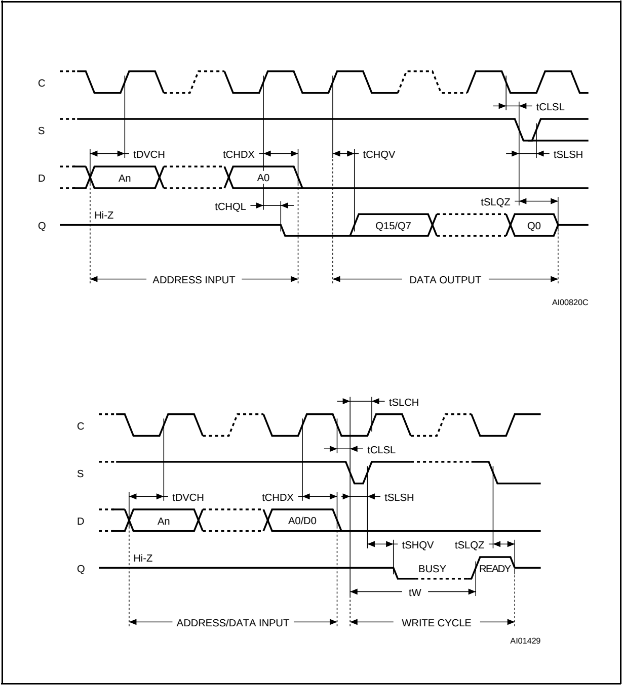
Figure 5. Synchronous Timing, Read or Write
