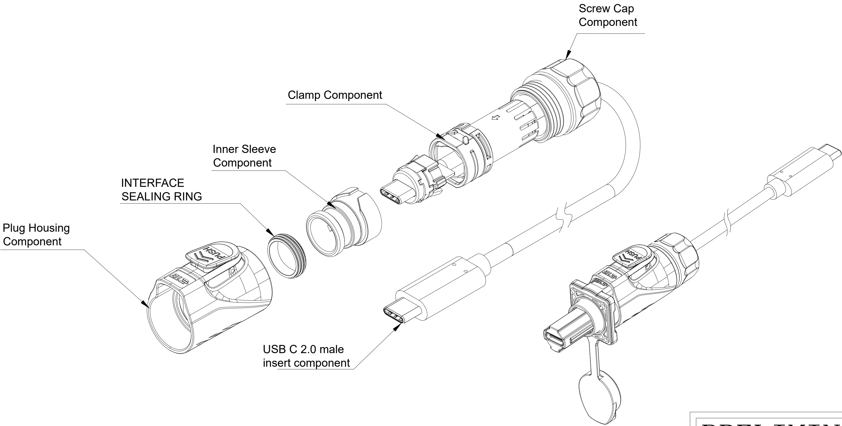
PLUG-RECEPTACLE ASSEMBLY
