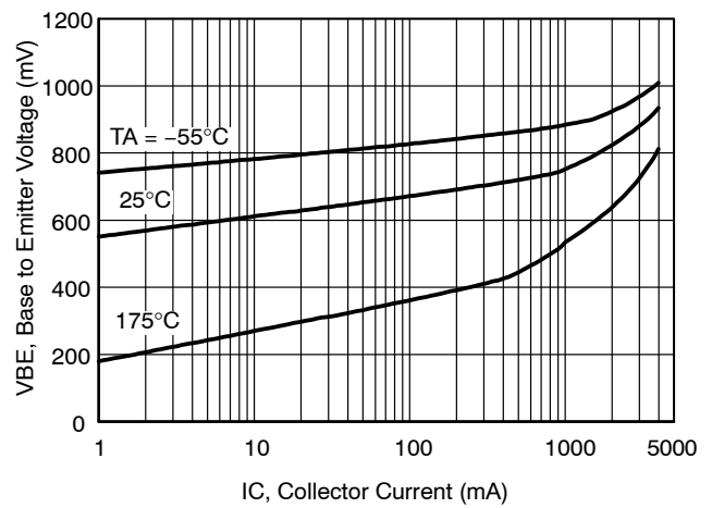
Figure 3. V_{BE} - I_C
